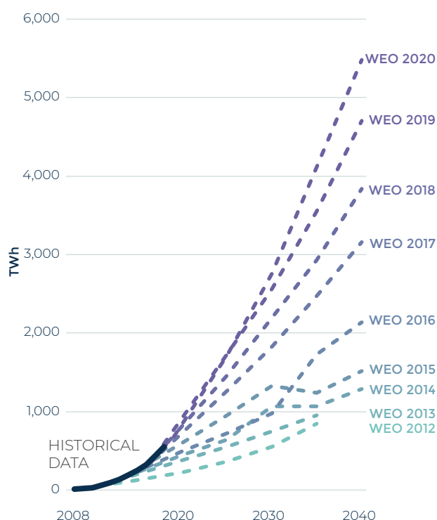
FIGURE 3. The International Energy Agency’s Stated Policies Scenarios have not accounted for the possibility of rapid, nonlinear growth in solar photovoltaic
