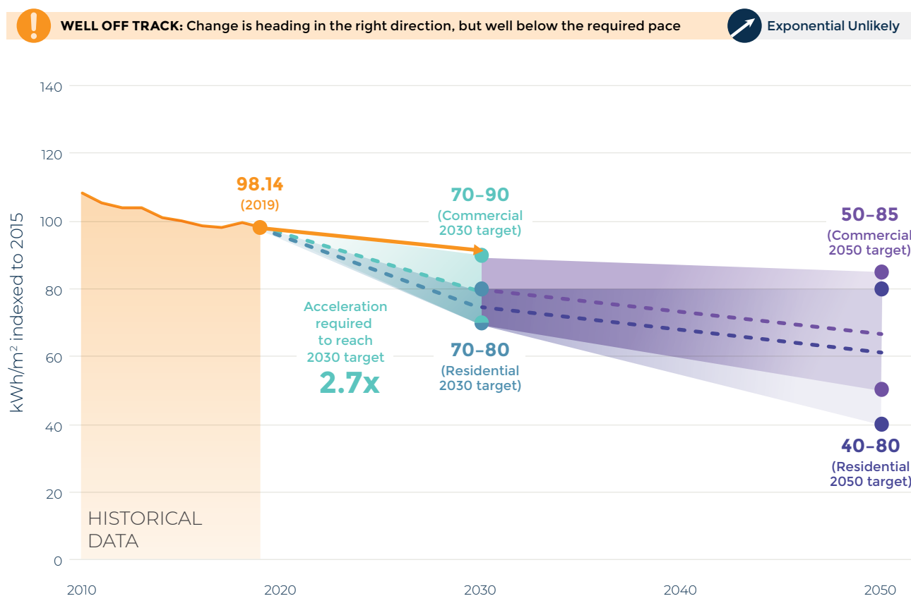
FIGURE 16. Historical progress toward 2030 and 2050 targets for energy intensity of building operations
